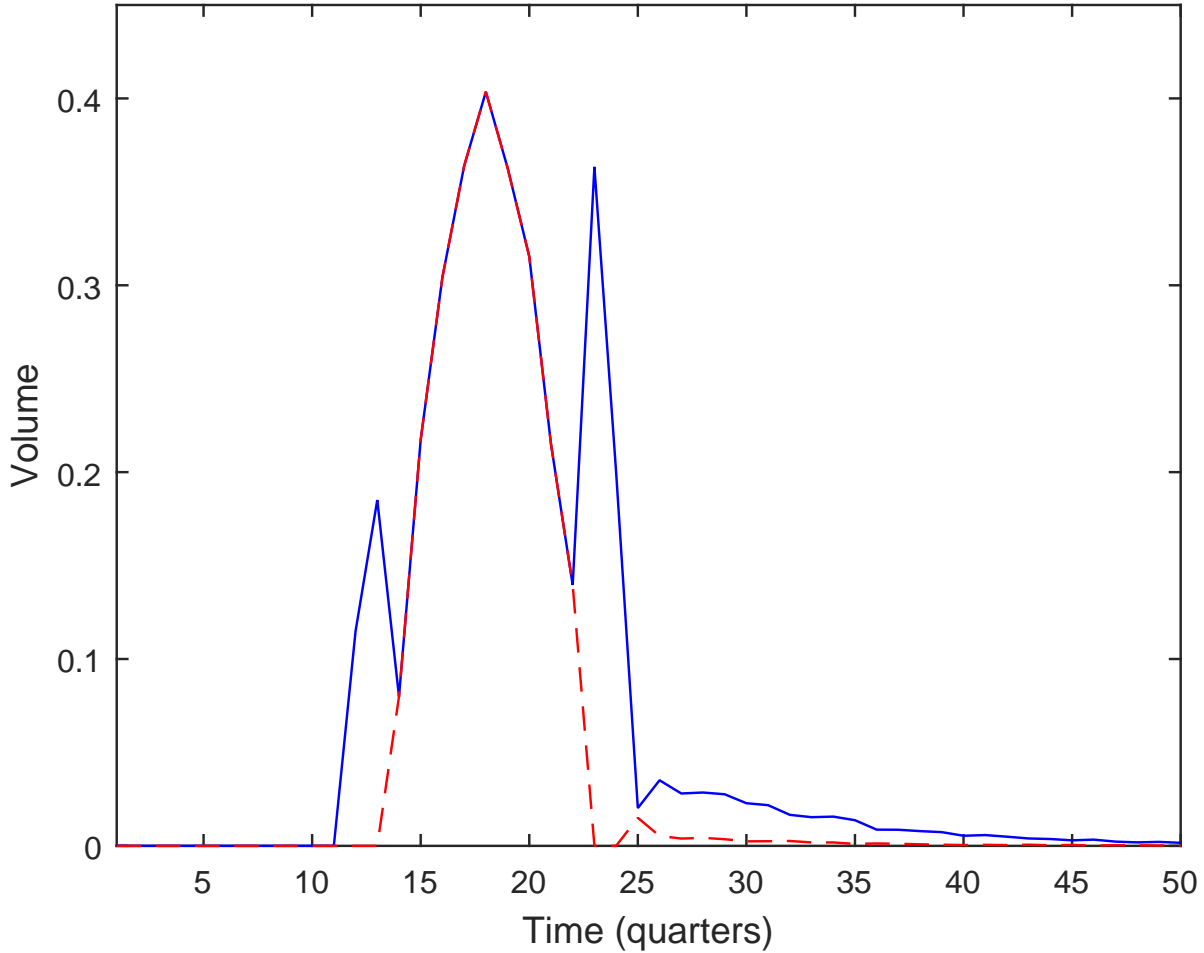
Fig. 5. Volume in a bubble. The solid line plots the total trading volume in the risky asset for the following sequence of 50 cash-flow shocks: 10 shocks of zero, followed by shocks of 2, 4, 6, 6, followed by 36 shocks of zero. The dashed line plots the trading volume between the extrapolators for the same cash-flow sequence. 30% of the investors are fundamental traders; the remainder are extrapolators with an extrapolation parameter \theta of 0.9 and who also put a base weight \bar{w}_i = 0.1 on a value signal. The other parameters are D_0 = 100 , T = 50 , \sigma_\varepsilon = 3 , Q = 1 , \gamma = 0.1 , \sigma_u = 0.03 , and I = 50 .
